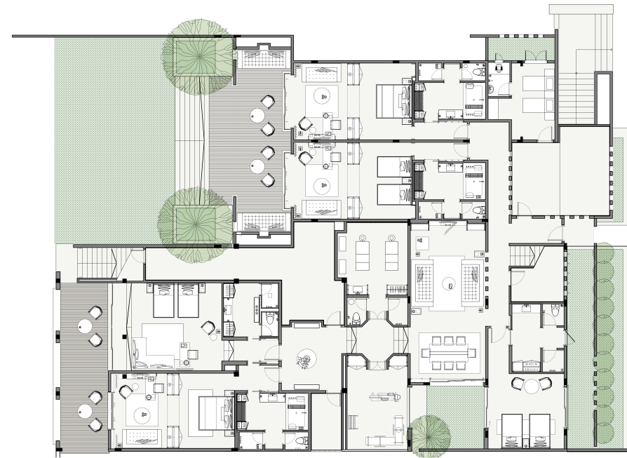
LOWER FLOOR 4 BEDROOMS
